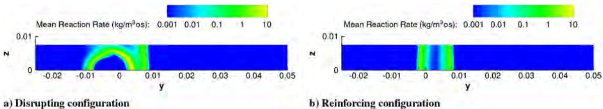
Fig. 4 Reaction-rate; slice 95% along cavity.
