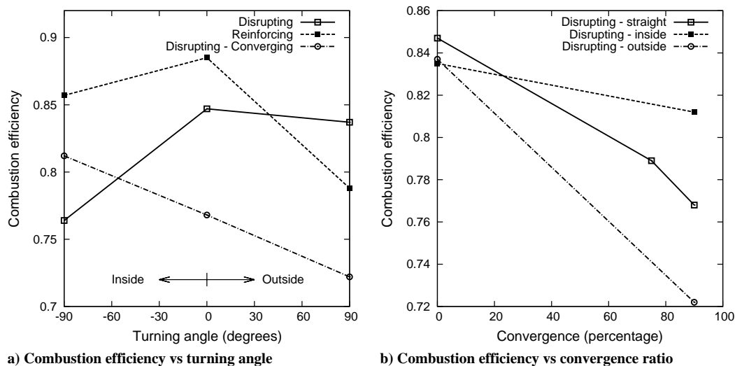
Fig. 16 Summary of combustion efficiencies.
